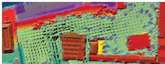
TUFLOW modelling of storm tide inundation from a hypothetical breach along the River Thames, London (courtesy Halcrow and the Environment Agency)
